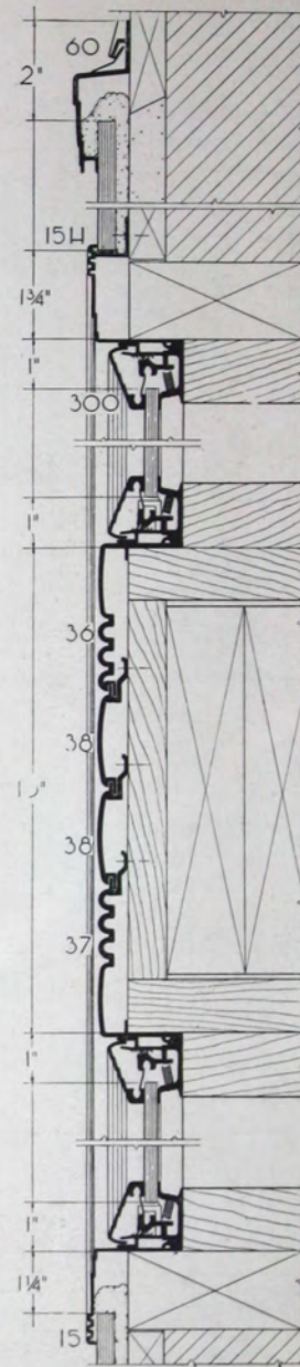
VERTICAL SECTIONS
