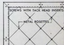
CEILINGS WITH BORDER IN RELIEF. VITROLITE MAY ALSO BE HELD WITH METAL MOULDINGS. MANY ARRANGEMENTS ARE POSSIBLE. SCALE 1/4"=1'-0"
