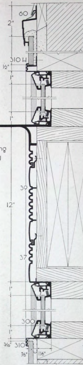
VERTICAL SECTIONS
