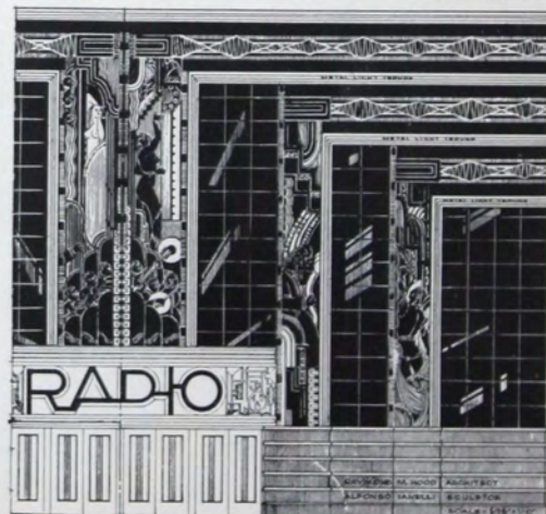
VITROLITE FACADE OF EXPOSITION BLDG. SHOWING USE OF VITROLITE WITH BAS-RELIEF SCULPTURE AND INDIRECT LIGHTING TROUGHES • SCALE 1/16"=1'-0"
