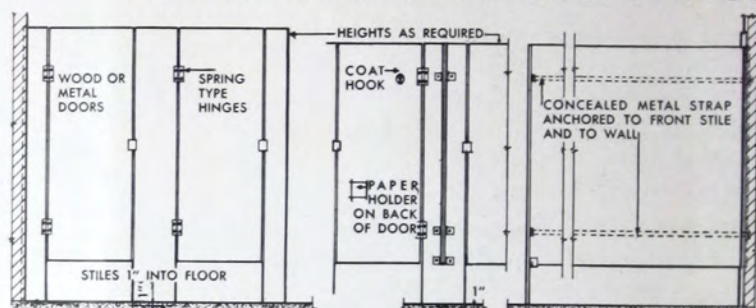
STANDARD TYPE USED IN THE FINEST OFFICE BUILDINGS. • SCALE 1/4"=1'-0"
