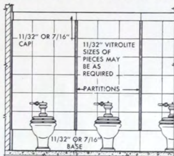
VITROLITE WAJNSCOTING AT BACK OF STALLS. SCALE 1/4"=1'-0"
