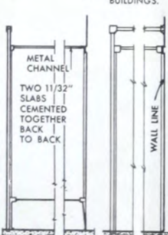
FRONT ELEVATION NEW TYPE OF VITROLITE TOILET STALL CONSTRUCTION WITH METAL HEADRAIL TO GIVE RIGIDITY AND WITH FLOATING PARTITION RELIEVED OF ALL STRAIN. SCALE 1/4"=1'-0"
