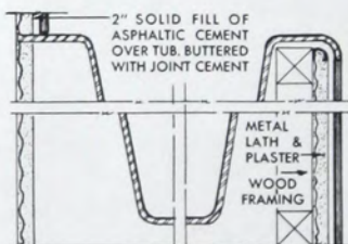
VITROLITE FACING ON TUBS PERMITS CARRYING UNIFORM BASE EFFECT AROUND ROOM. TUBS AS ABOVE SUPPLIED BY MOST BATHROOM FIXTURE MANUFACTURERS. SCALE 1 1/2"=1'-0"
