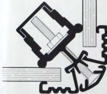
21 DIVISION BAR
