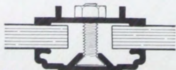
121 TRANSOM DIVISION BAR
