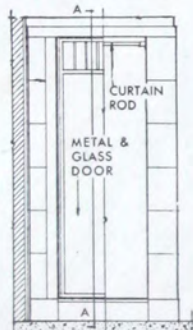
ELEVATION SCALE 1/4"=1'-0"
