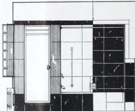
VITROLITE SCHEMES, SHOWER AND TUB RECESS SCALE 1/4"=1'-0"
