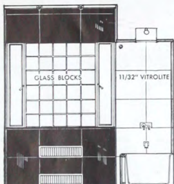
BATHROOM WALLS AND CEILING SCALE 1/4"=1'-0"
