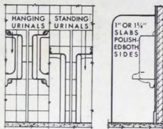
VITROLITE PARTITION SLABS AND WAJNSCOTING. SCALE 1/4"=1'-0"
