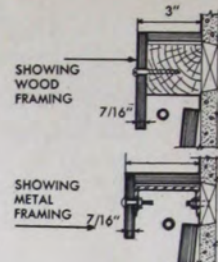
SECTIONS AT A-A SCALE 1/2"=1'-0"
