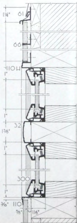
VERTICAL SECTIONS
