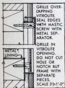
GRILLE DETAILS
