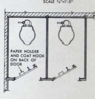
FLOOR PLAN WIDTH, DEPTH AND ARRANGEMENT TO SUIT REQUIREMENTS • SCALE 1/4"=1'-0"
