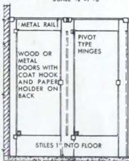
FRONT ELEVATION NEW TYPE OF VITROLITE TOILET STALL CONSTRUCTION WITH METAL HEADRAIL TO GIVE RIGIDITY AND WITH FLOATING PARTITION RELIEVED OF ALL STRAIN. SCALE 1/4"=1'-0"
