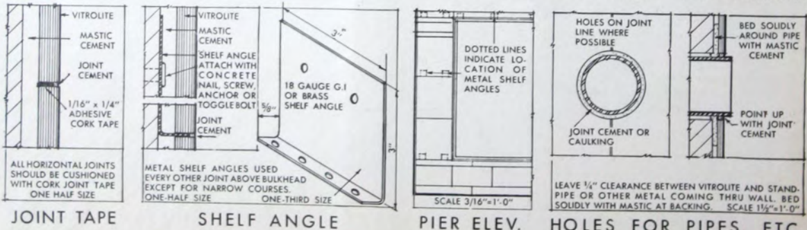
HOLES FOR PIPES, ETC.
