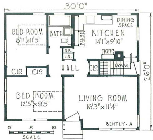
PLAN A, FOR LOW PITCH ROOF
