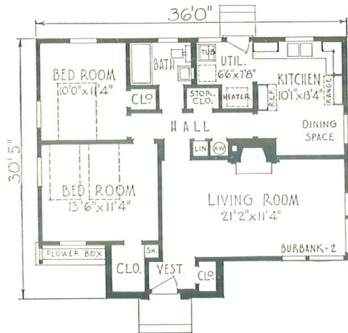
PLAN 2, WITHOUT BASEMENT
