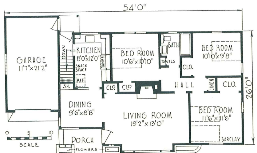
ALTERNATE DESIGN B — BRICK CONSTRUCTION
