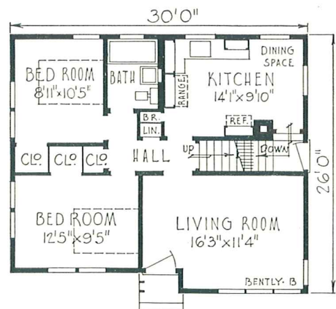
PLAN B, PROVIDING ATTIC SPACE
