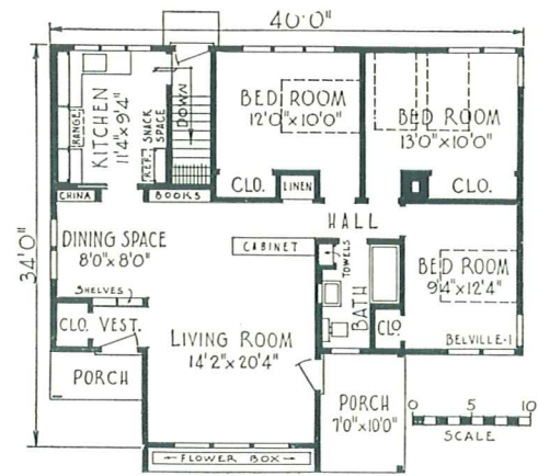
PLAN 1, WITH BASEMENT
