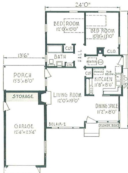
PLAN 2, WITHOUT BASEMENT
