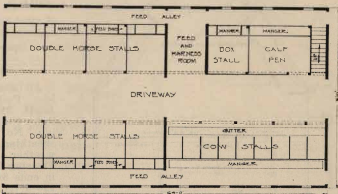
THE HOLSTEIN GOTHIC BARN—36x64—12' Studs (See specifications below)
