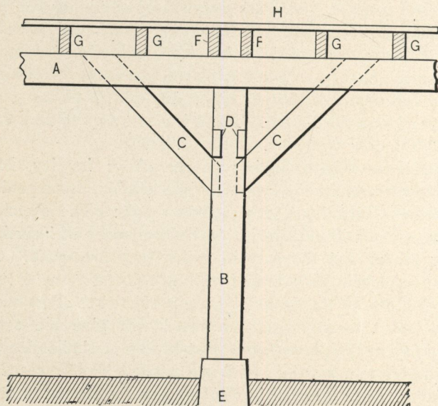
Fig. 1.—Showing Method of Bracing.
