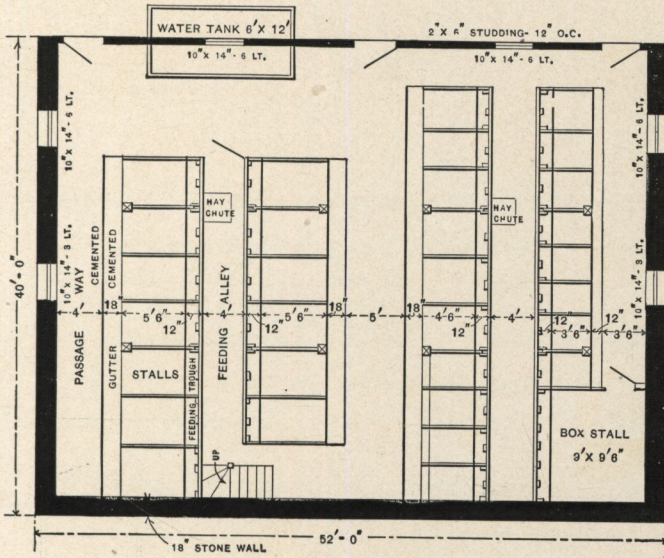
Basement Plan.—Scale, 1-16 Inch to the Foot.
