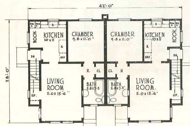
PLAN No. D-4100 Size 42'-0" x 28'-0" — Area 1095 sq. ft. This duplex cottage was designed for investment property and provides a basement and attic space for the use of both families.
