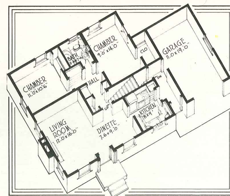
FLOOR PLAN NO. 4423 SIZE 45'-0" x 28'-0"
