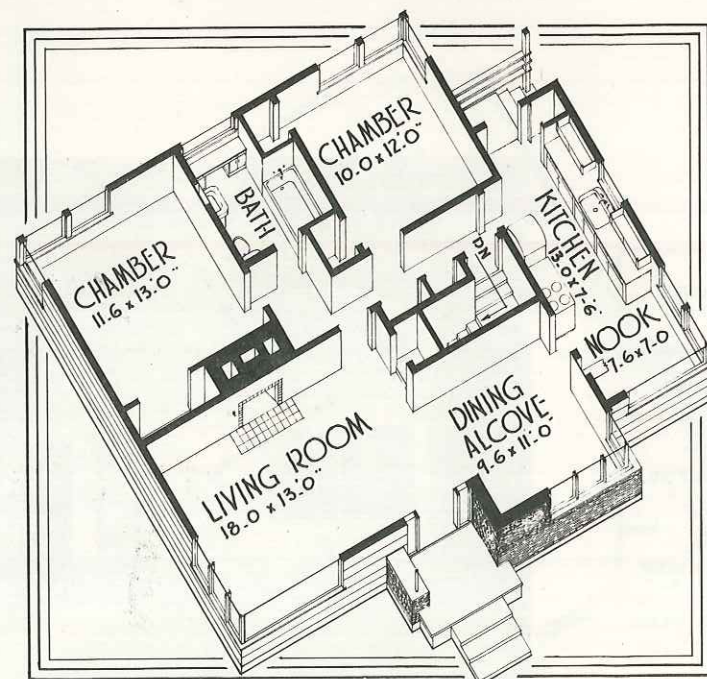
FLOOR PLAN NO 5139 SIZE 37'-0" x 30'-0"
