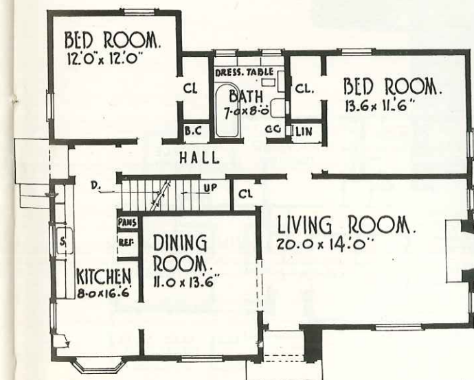
PLAN No. 5026 Size 41'-0" x 34'-0" — Area 1237 sq. ft. A variation of the Cape Cod type, this home was designed for comfort and provides a large attic and full basement.
