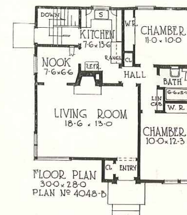
PLAN No. 4048-B Size 30'-0" x 28'-0" — Area 910 sq. ft. This modern house was designed especially for the small family for an average city lot. A playroom may be built in the large basement.
