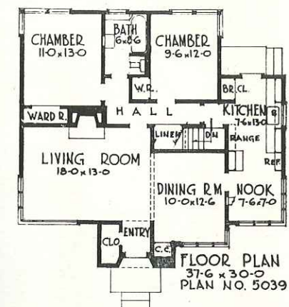
PLAN No. 5039 Size 37'-6" x 30'-0" — Area 1128 sq. ft. A tremendous amount of light is furnished by the larger corner windows in this house which has a partitioned full basement.
