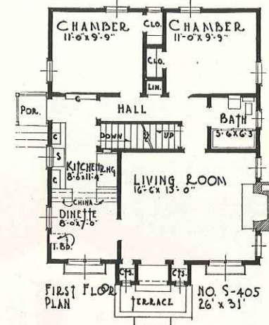
PLAN No. S-405 Size 26'-0" x 31'-0" — Area 818 sq. ft. The English style exterior of this shake finished house provides an attic which can be finished into additional sleeping rooms.
