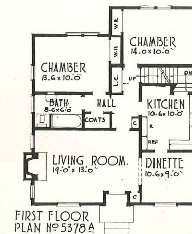
PLAN No. 5378-A Size 31'-0" x 36'-0" — Area 1046 sq. ft. Like all Cape Cod Cottages, this one takes advantage of every bit of available space and provides a breakfast table in the kitchen.
