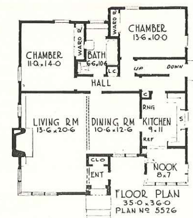
PLAN No. 5526 Size 35'-0" — 36'-0" — Area 1235 sq. ft. A fine, convenient floor plan is shown here in modernistic dress that permits a large attic for future use and a full size basement.
