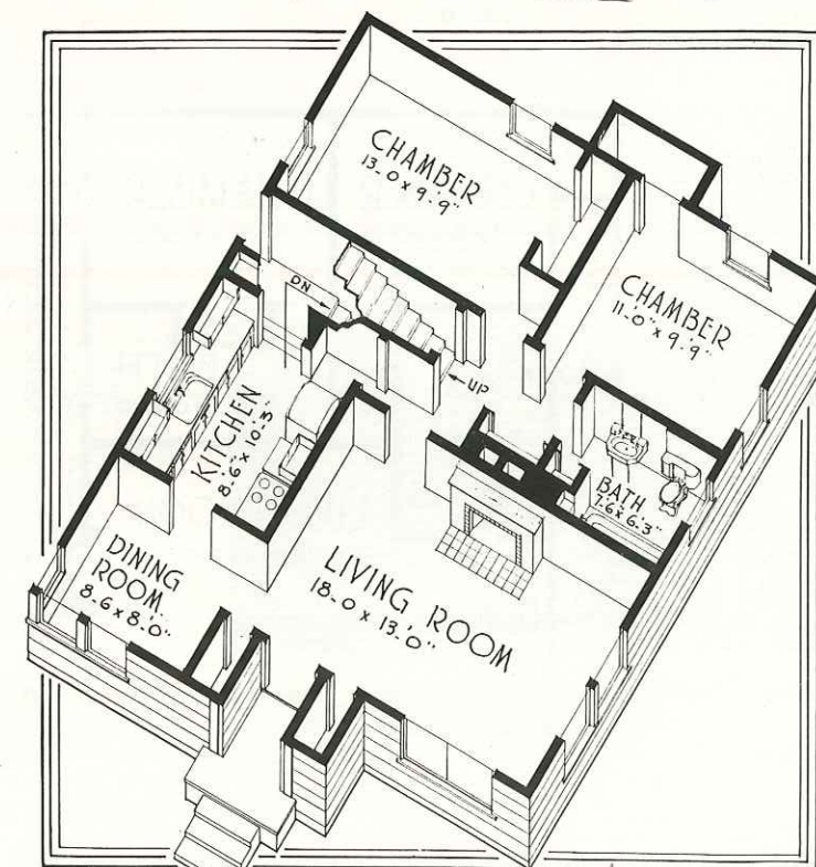
FLOOR PLAN NO 5678 SIZE 28'-0" x 35'-0"
