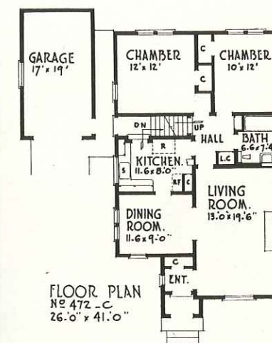
PLAN No. 472-C Size 26'-0" x 41'-0" — Area 1018 sq. ft. An interesting form of the modernized Early American type, this home provides a large attic for future bedrooms and a full basement.
