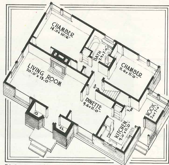
FLOOR PLAN No 5188 SIZE - 44'-0" x 27'-0"
