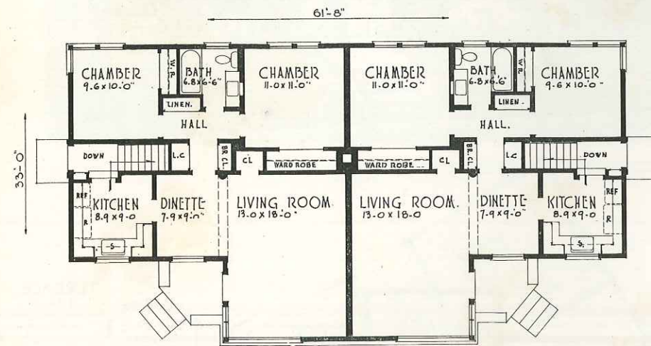
PLAN No. D-4060 Size 61'-8" x 33'-0" Area 1729 sq. ft. This streamlined duplex house was designed for a corner lot and to give a maximum comfort to families occupying either side.
