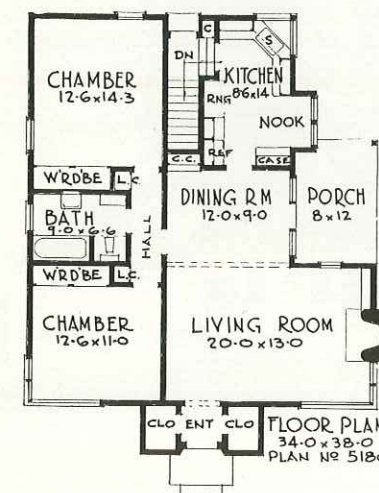
PLAN No. 5180 Size 34'-0" x 38'-0" — Area 1179 sq. ft. One of the charming features of this modern home is the side porch which can be used as family entrance or outdoor dining room.
