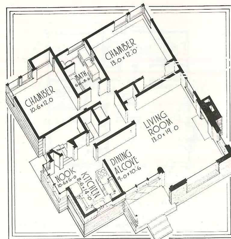
FLOOR PLAN No 5726 SIZE 32.0 x 35.0
