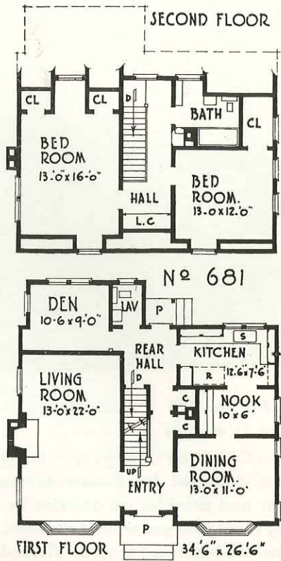
PLAN No. 681 Size 34'-6" x 26'-6" — Area 1012 sq. ft. An unusual New England Colonial style, this house has many advantages in arrangement, and has imposing appearance.
