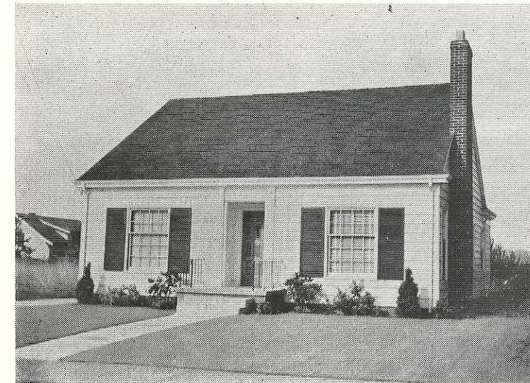
PLAN No. 5031 Size 32'-0" x 41'-0" — Area 1208 sq. ft. This large Cape Cod Cottage has space in the attic for two additional bedrooms and a bath to take advantage of space.
