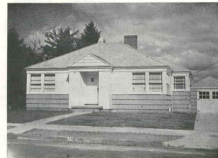
PLAN No. 4356 Size 32'-0" x 26'-0" — Area 896 sq. ft. Shakes on the lower portion with a belt of vertical boards at window height give this convenient house its streamlined appearance.
