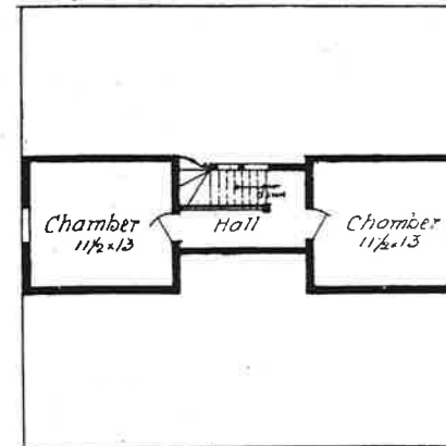
Second Floor Plan V. W. Voorhees Archt Seattle Wash
