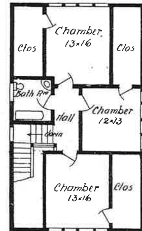
Second Floor Plan V.W. Voorhees Architect Seattle No 131
